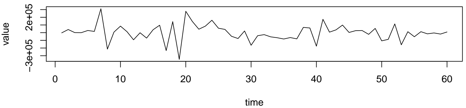
Working Time Series ( \lambda=1, d=0, D=1 )
