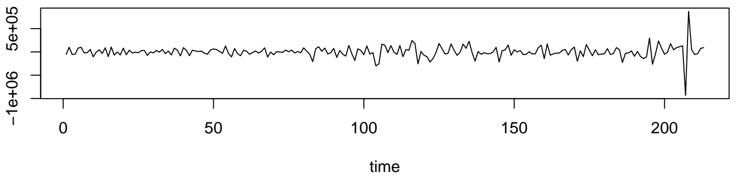
Working Time Series (lambda=1, d=1, D=1)
