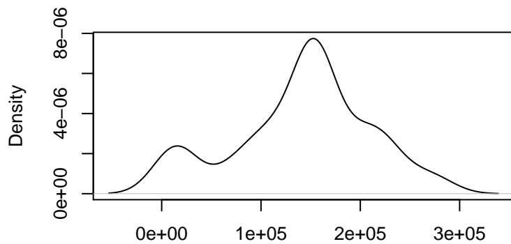
Kernel Density Plot of Predictions
