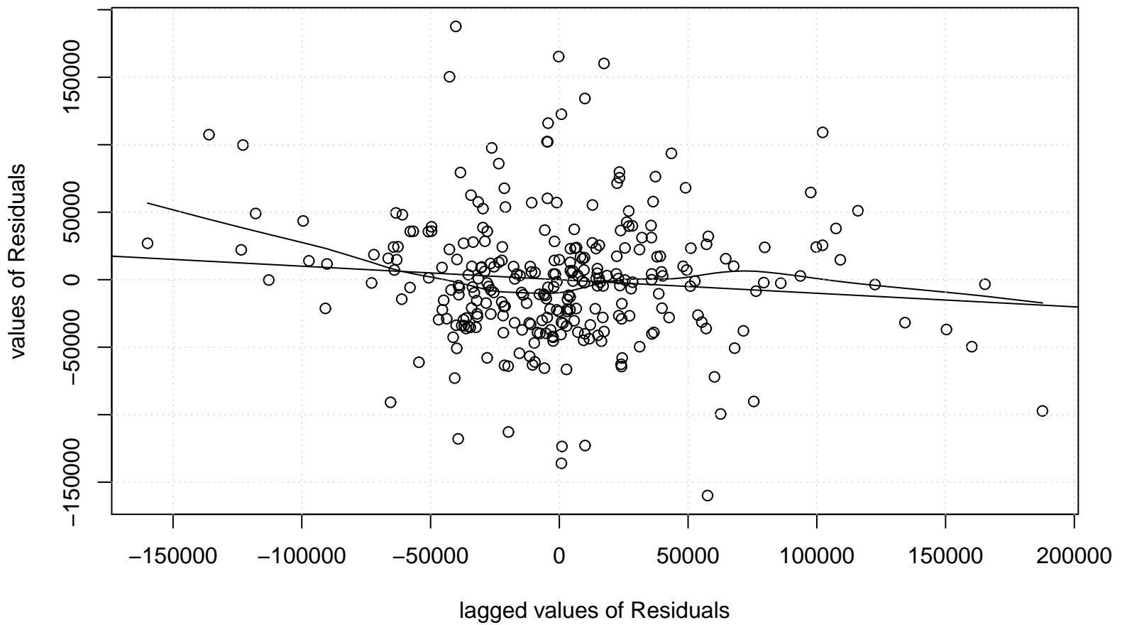
Residual Lag plot, lowess, and regression line
