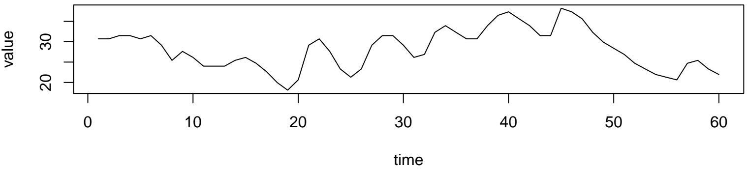
Working Time Series (lambda=2, d=0, D=0)
