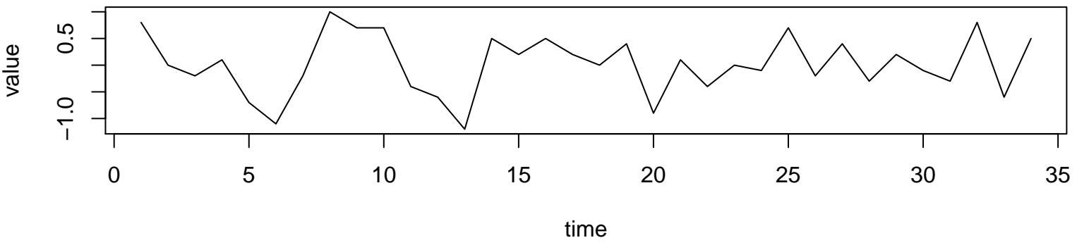
Working Time Series (lambda=1, d=2, D=2)
