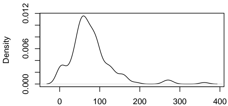
Kernel Density Plot of Actuals
