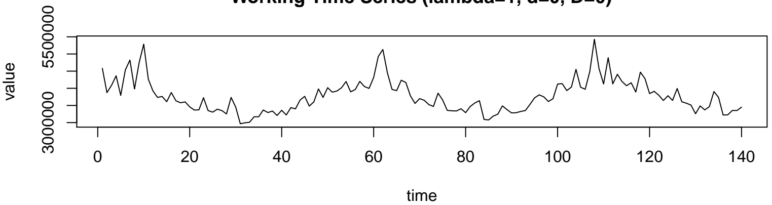
Working Time Series ( \lambda=1, d=0, D=0 )
