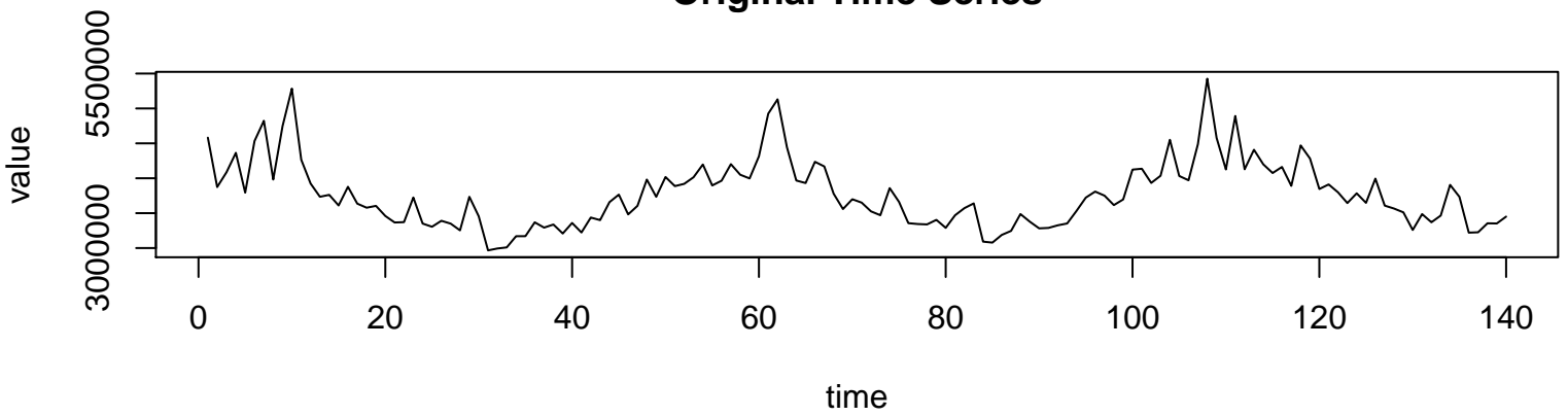
Original Time Series
