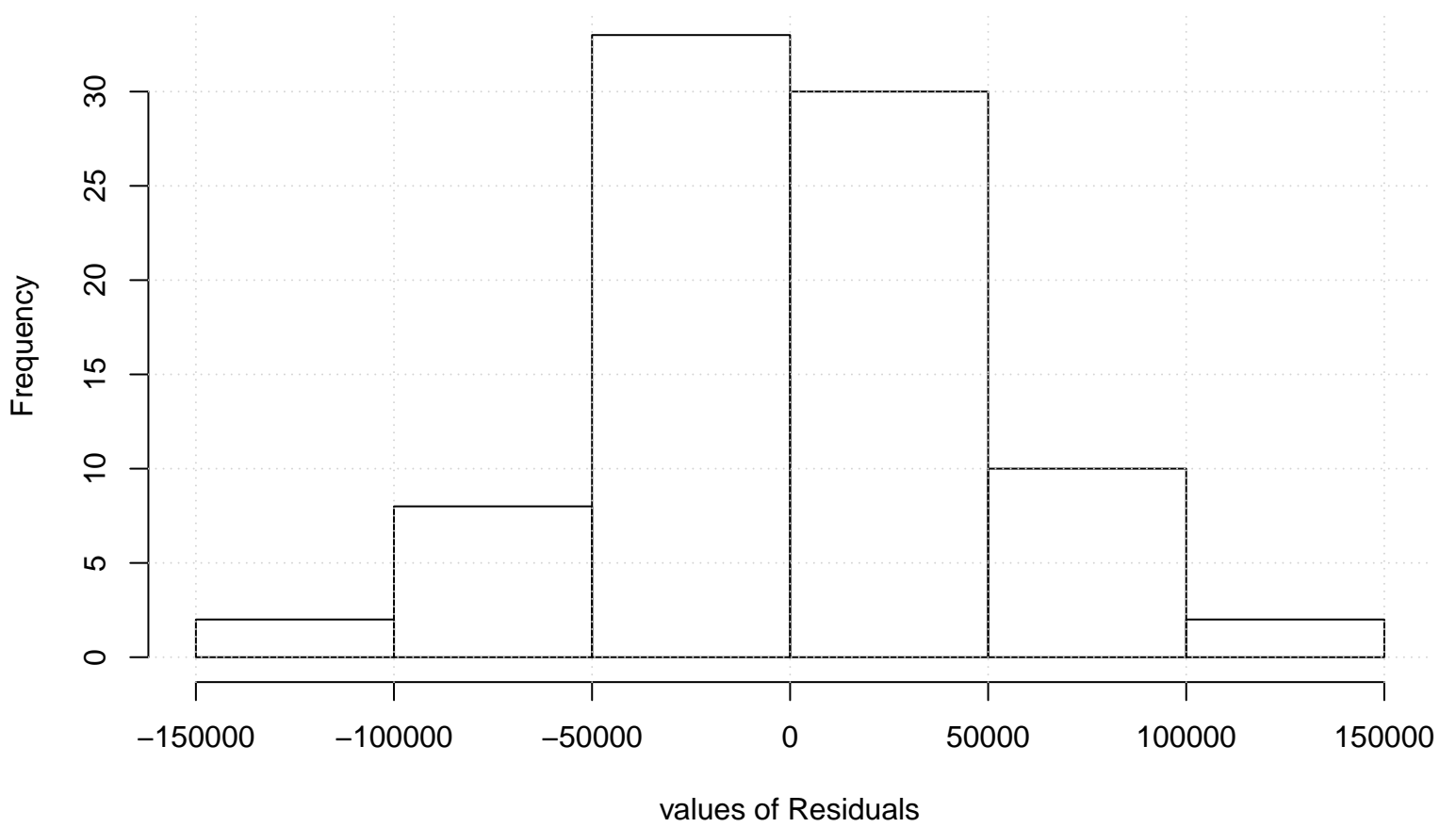
Residual Histogram
