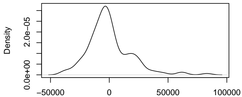
Kernel Density Plot of Residuals
