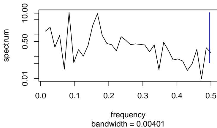
Standardized Residuals
