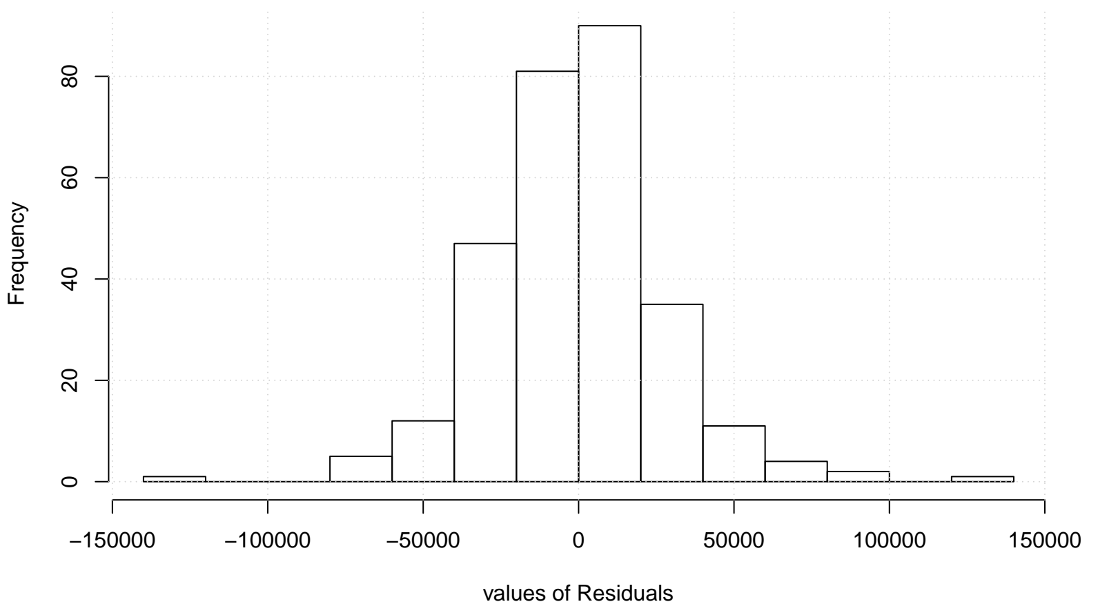
Residual Histogram
