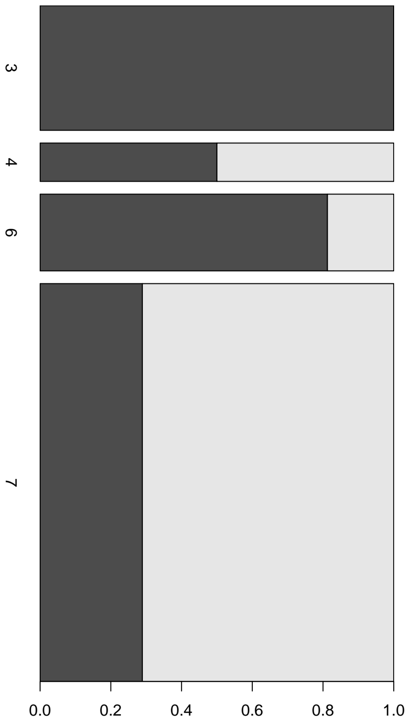
Response by Terminal Node
