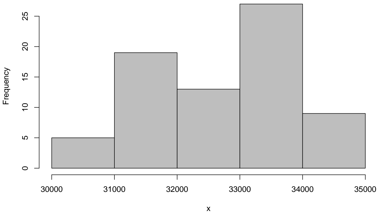
Histogram
