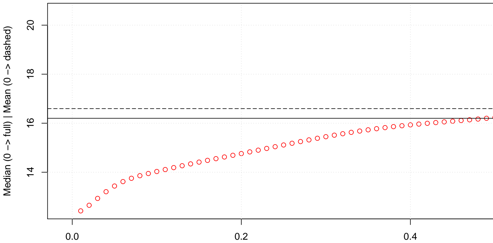
Harrell-Dav
