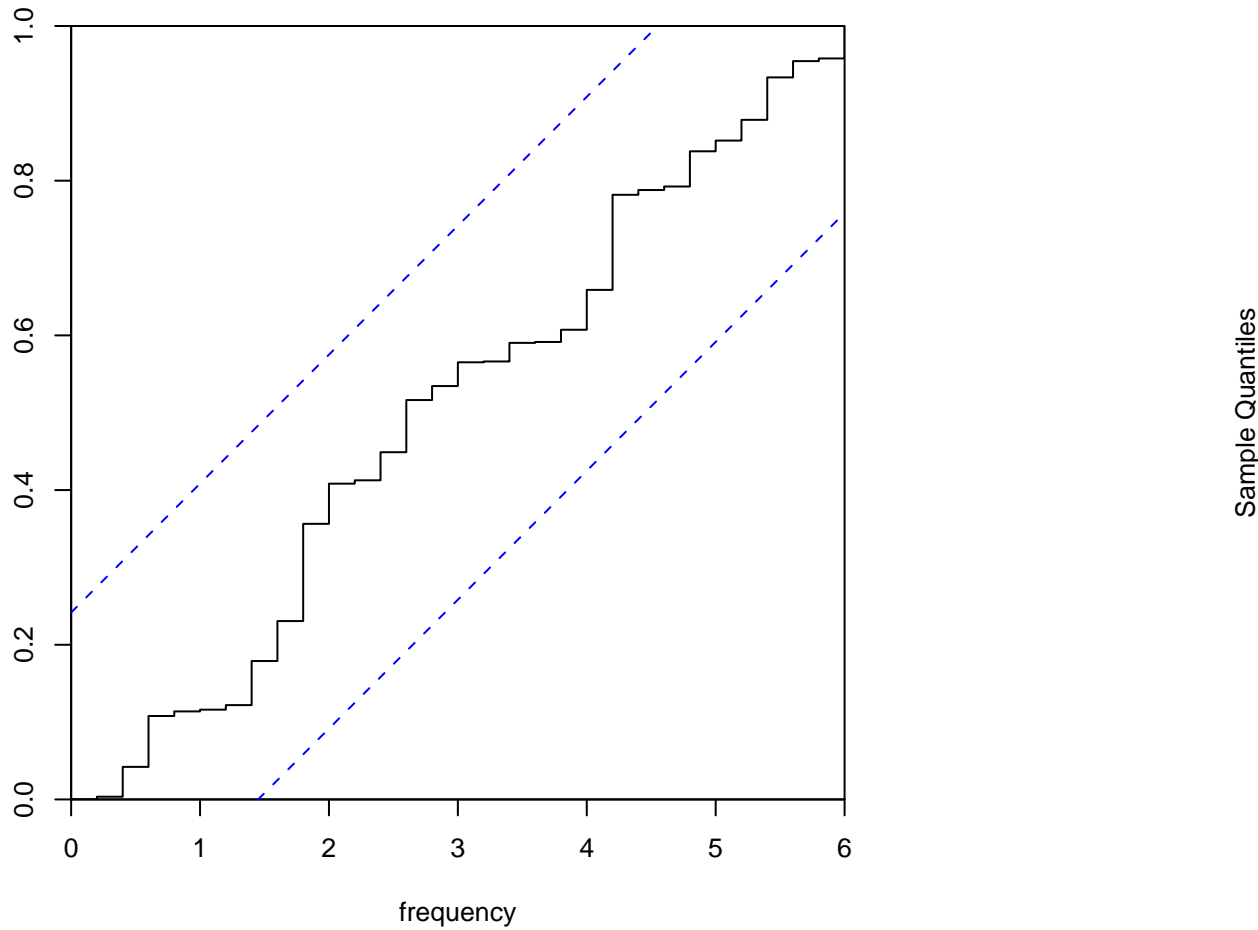
Residual Cumulative Periodogram
