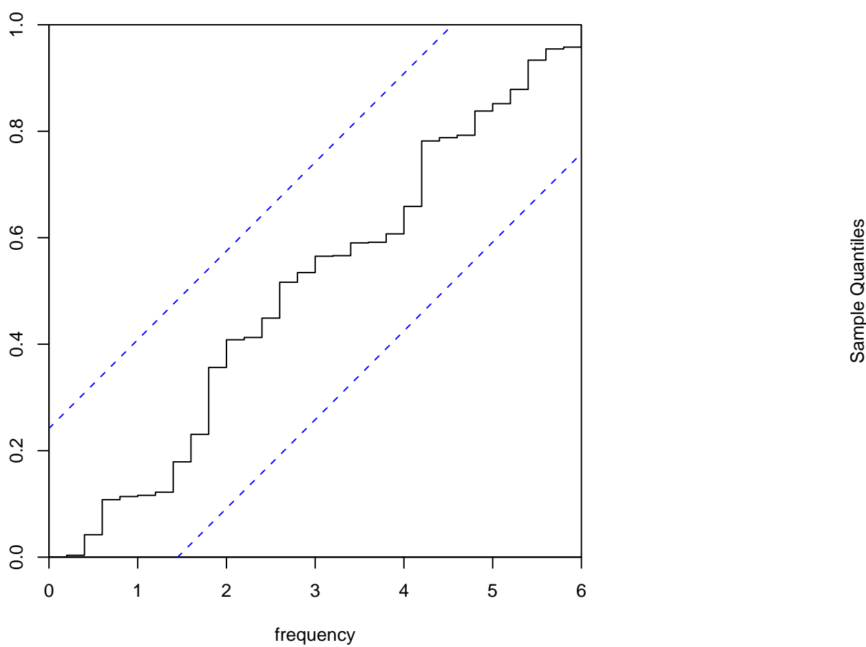
Residual Cumulative Periodogram
