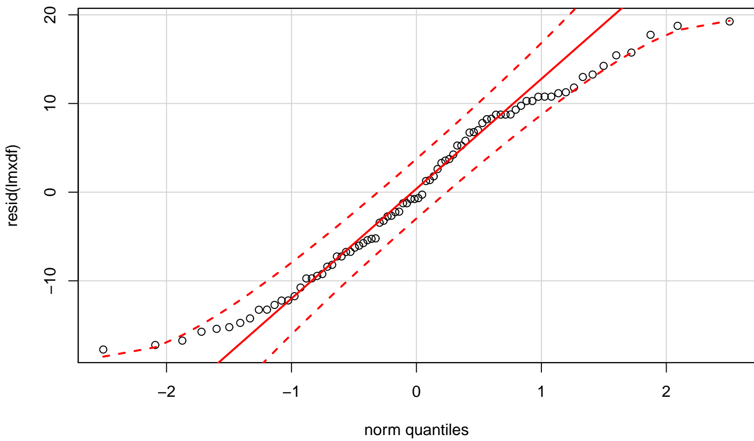
QQplot of Residuals of Fit
