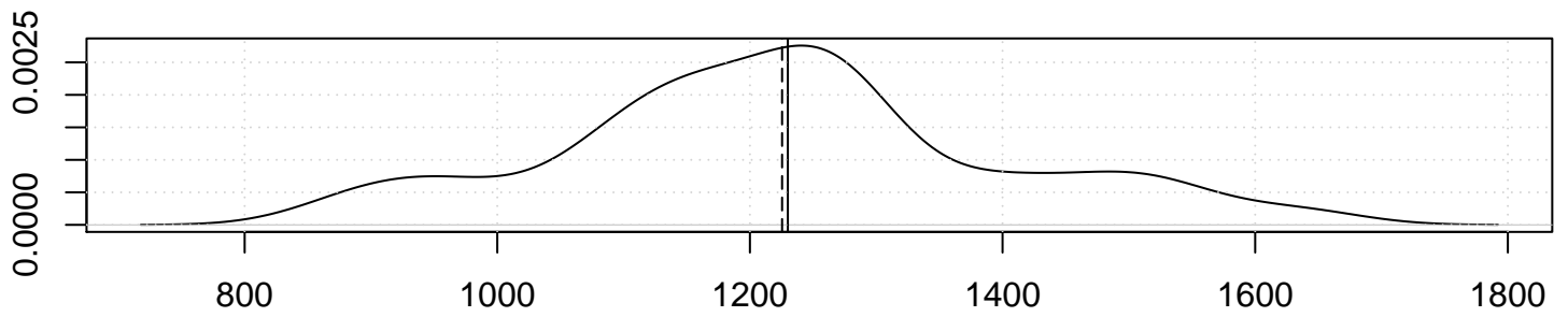
Density Plot – Gaussian Kernel
