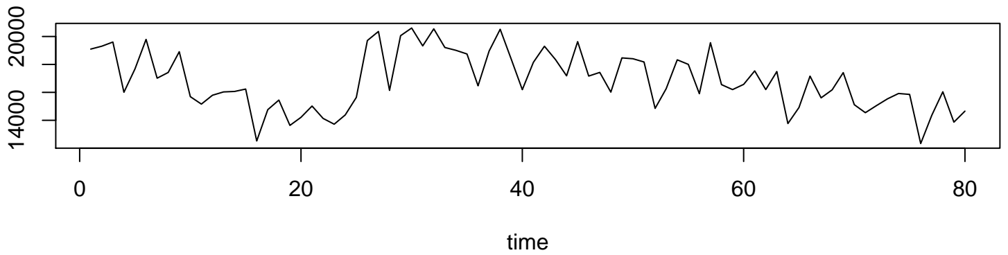
Original Time Series
