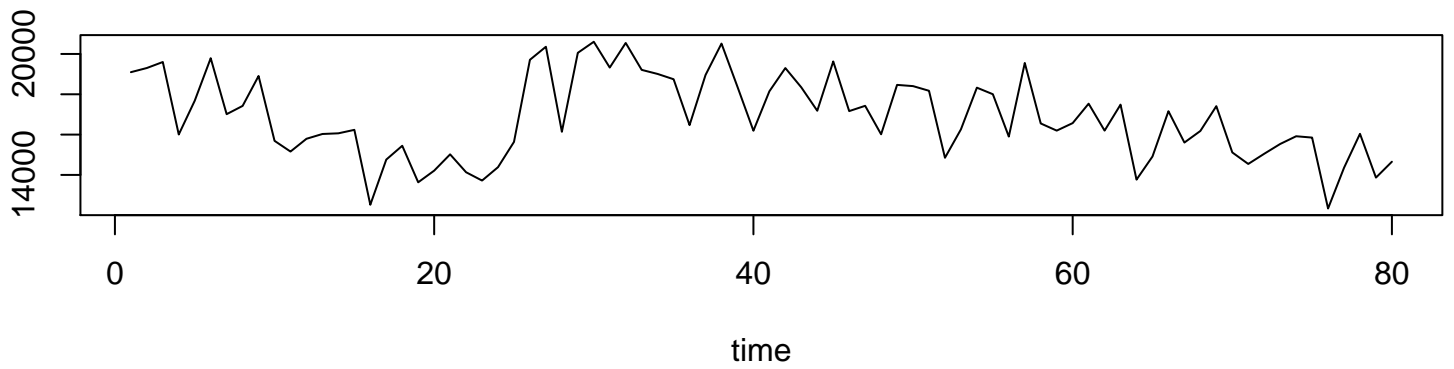
Working Time Series (lambda=1, d=0, D=0)
