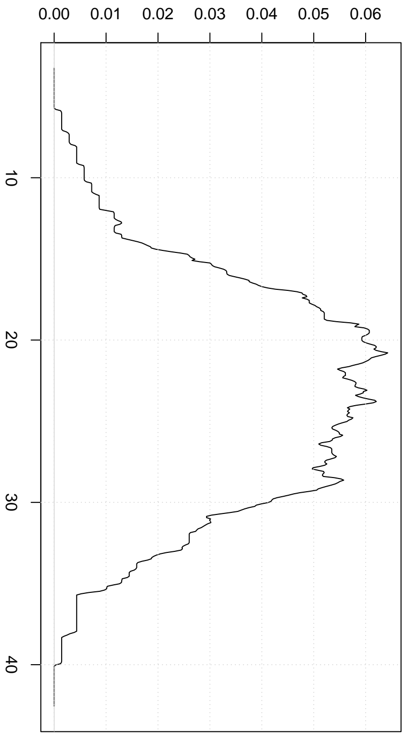
Rectangular Kernel
