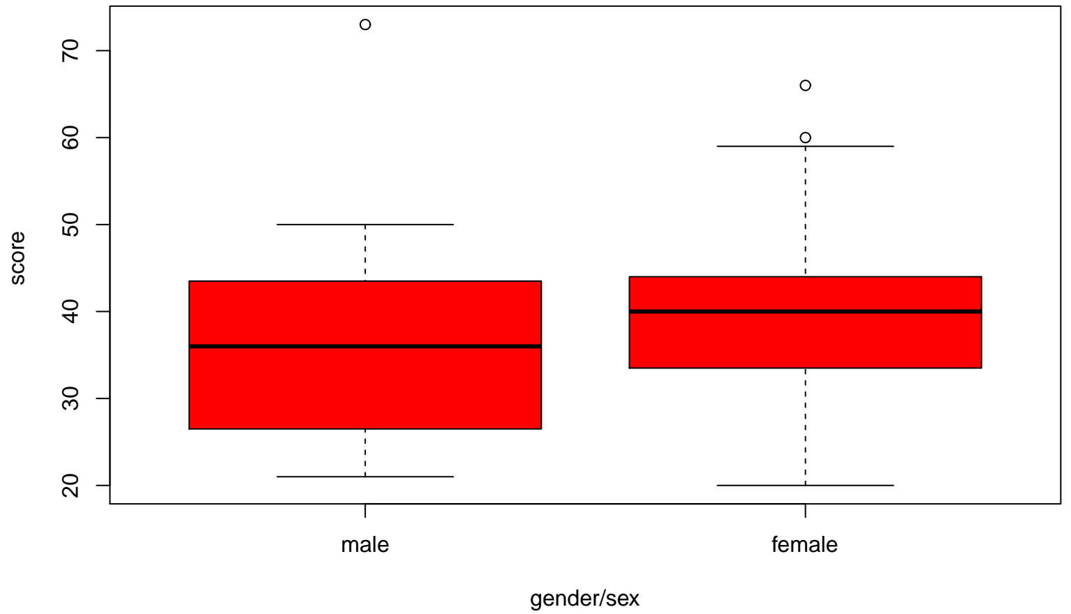
bpvt distribution
