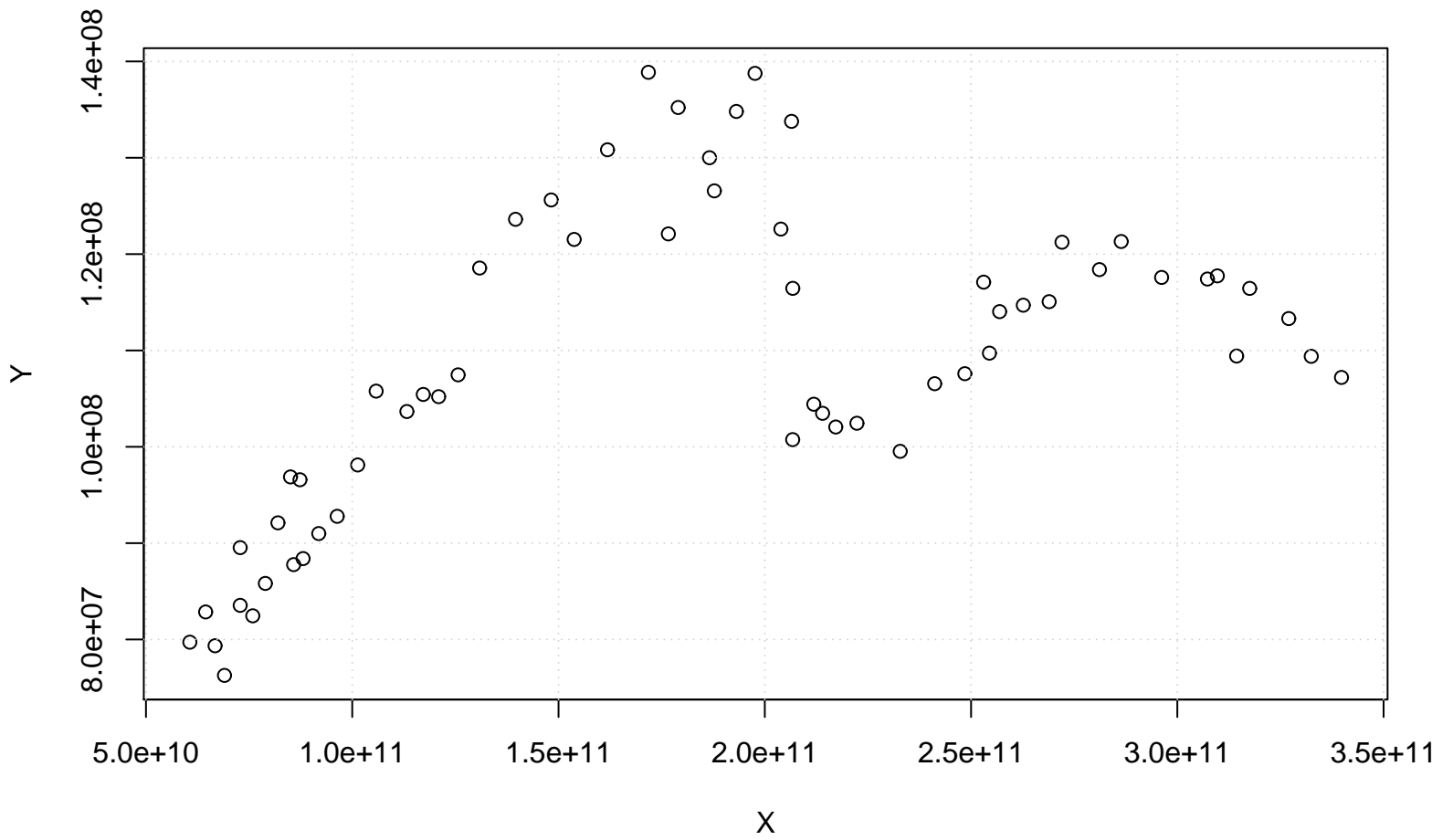
Scatterplot
