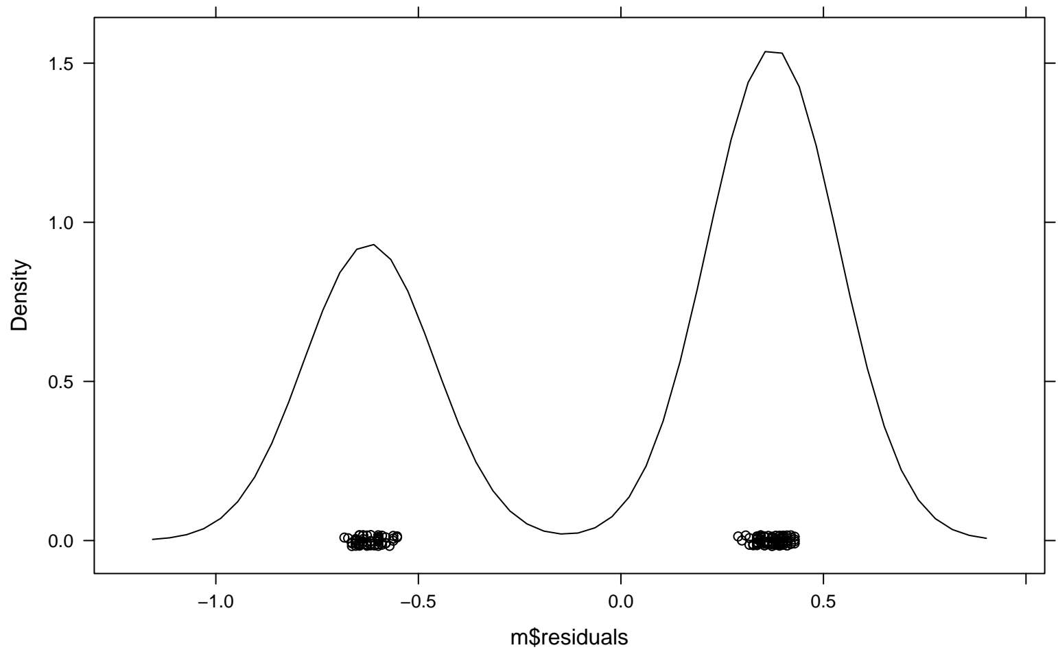
Density Plot
