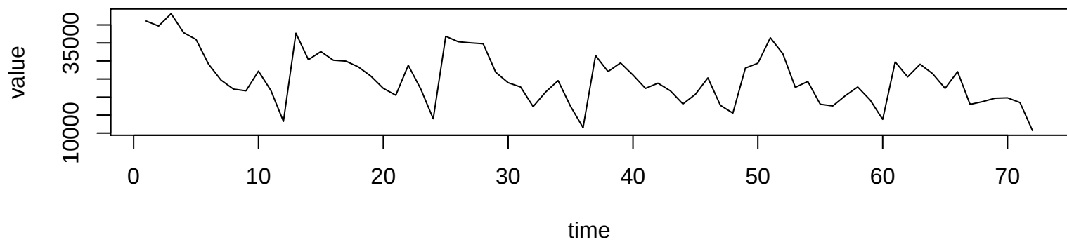
Original Time Series
