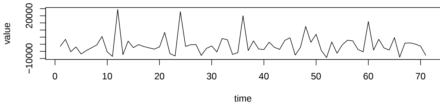
Working Time Series ( \lambda=1 , d=1 , D=0 )
