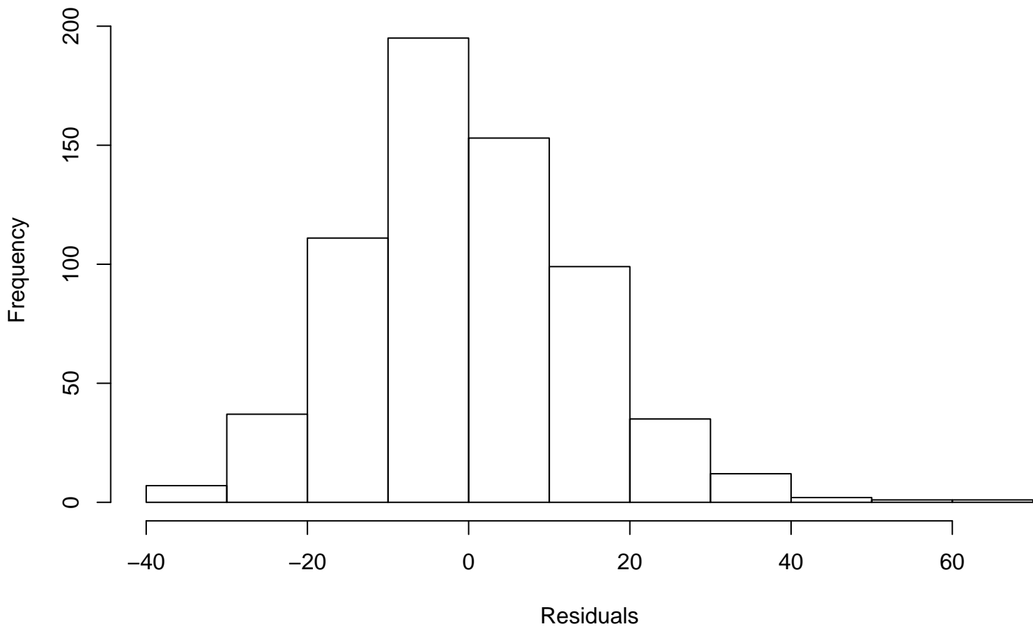
Residual Histogram
