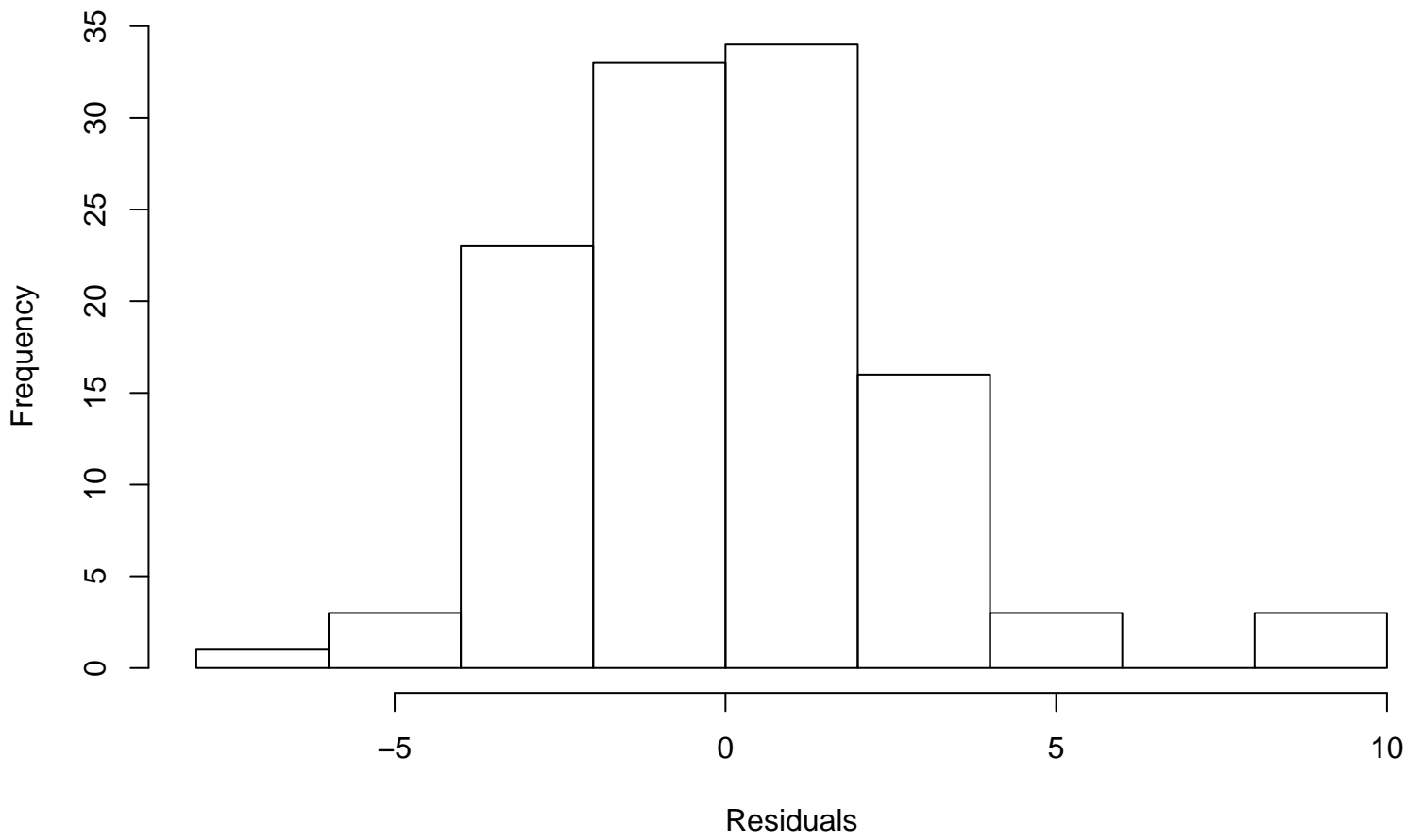
Residual Histogram
