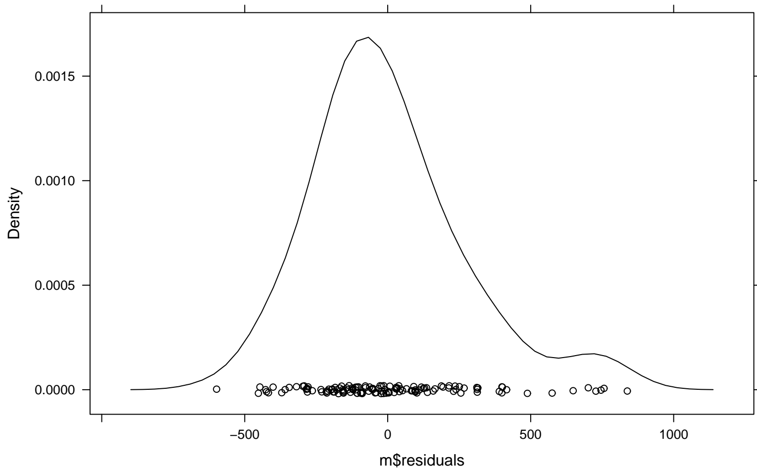
Density Plot bw = 100
