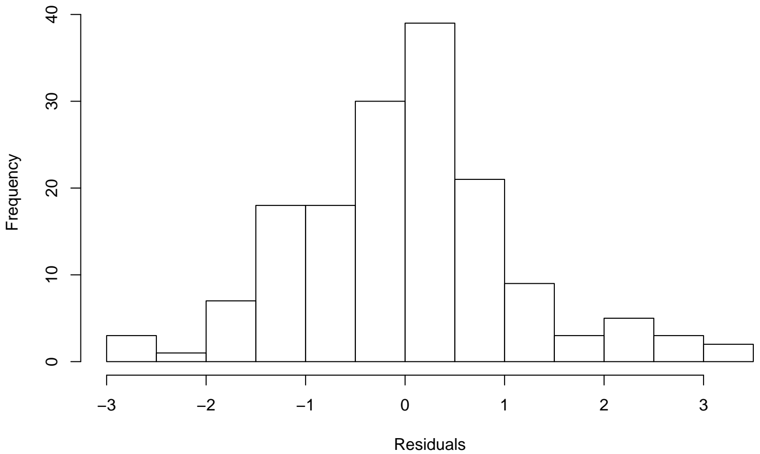
Residual Histogram
