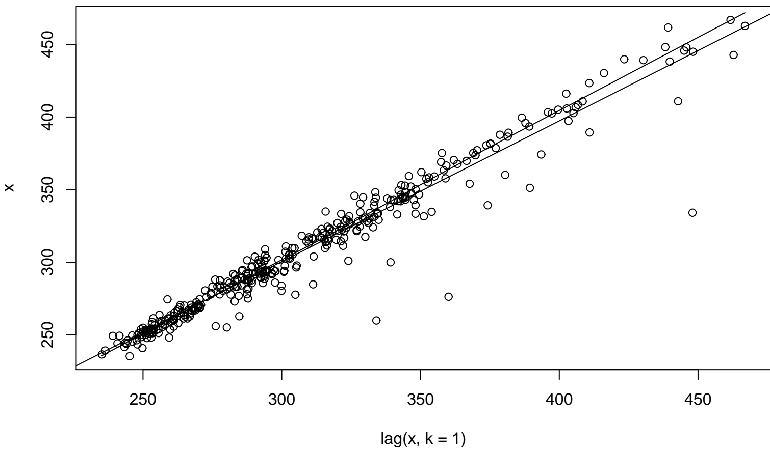
Lag plot, lowess, and regression line
