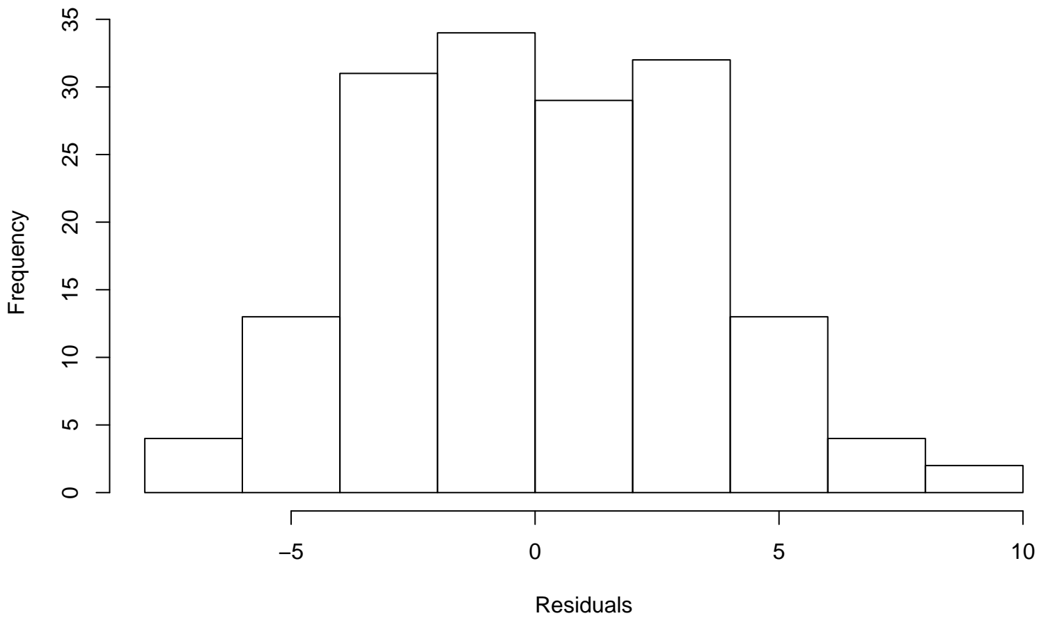
Residual Histogram
