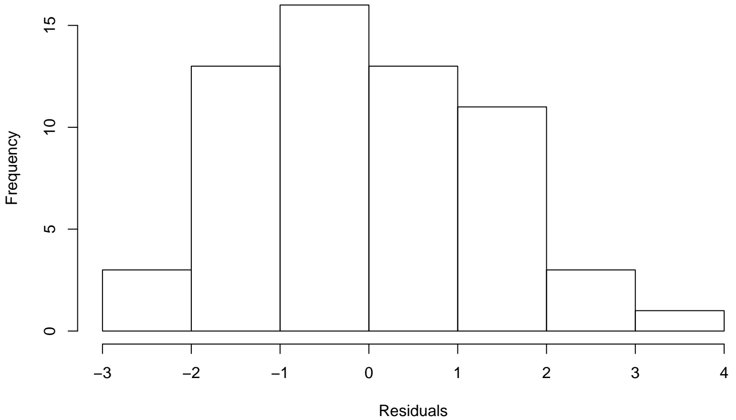
Residual Histogram
