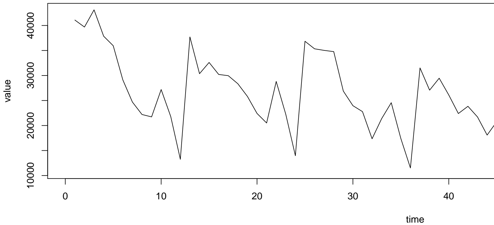
Working Time Series ( \lambda=1, d=0 )
