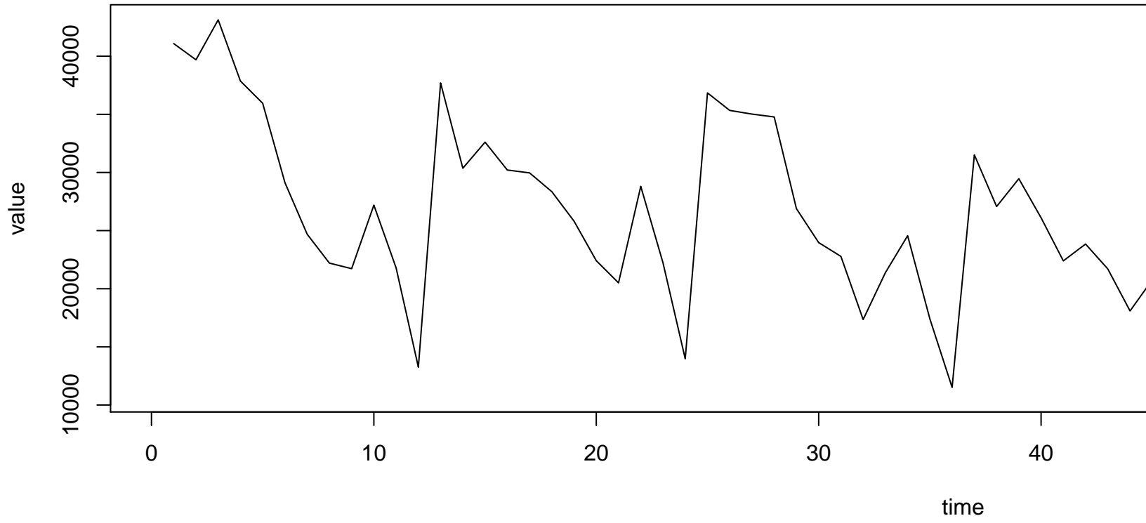
Original Time Series
