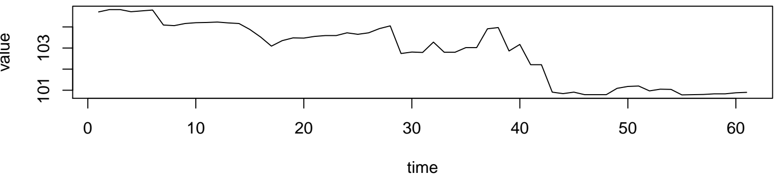
Working Time Series (lambda=1, d=0, D=0)
