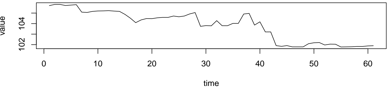
Original Time Series
