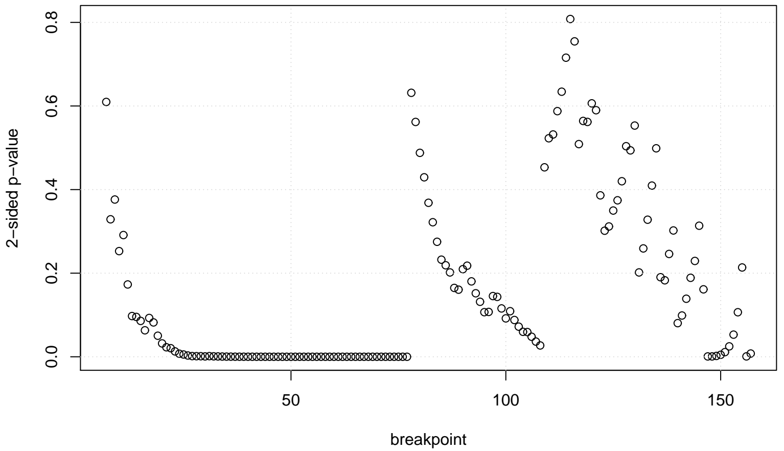
Goldfeld-Quandt test
