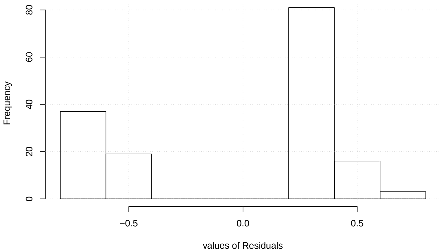
Residual Histogram
