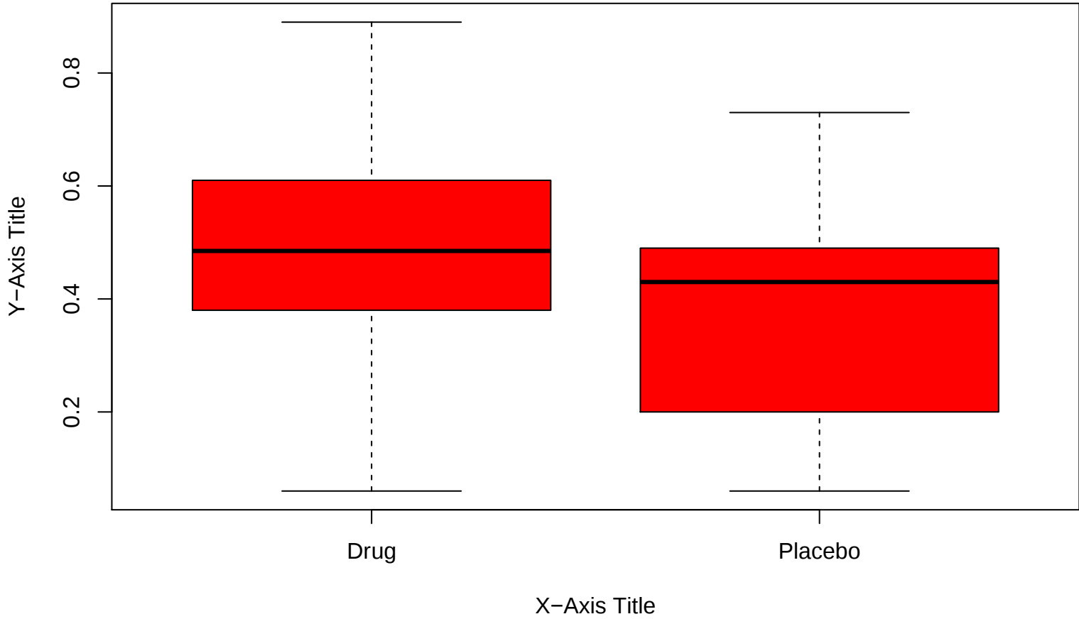
Boxplots Title
