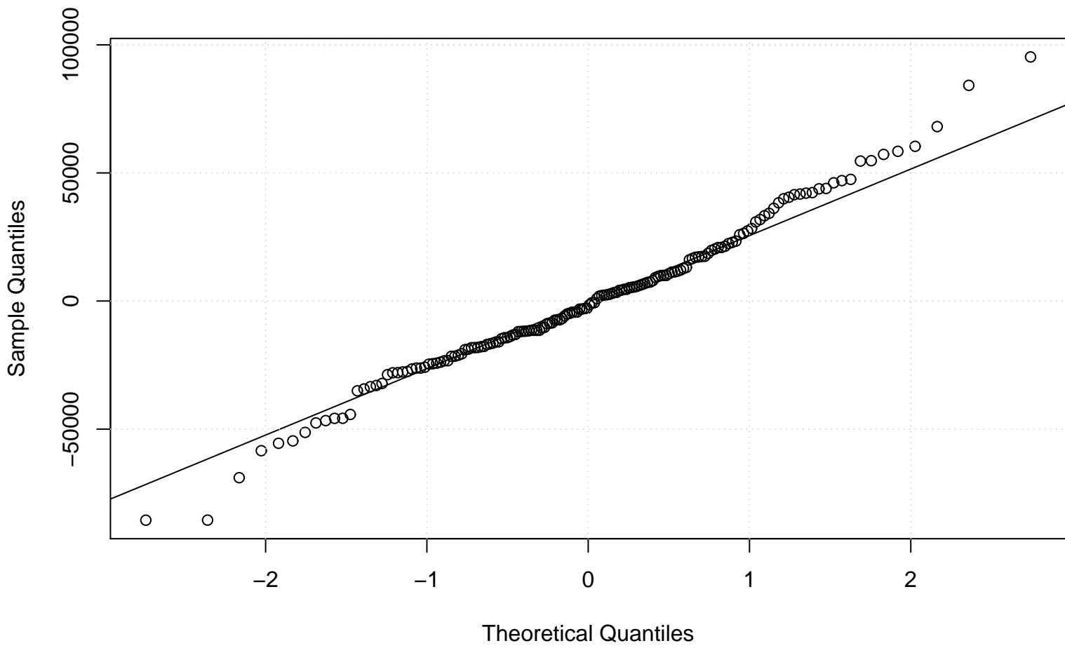
QQ plot of e[t]
