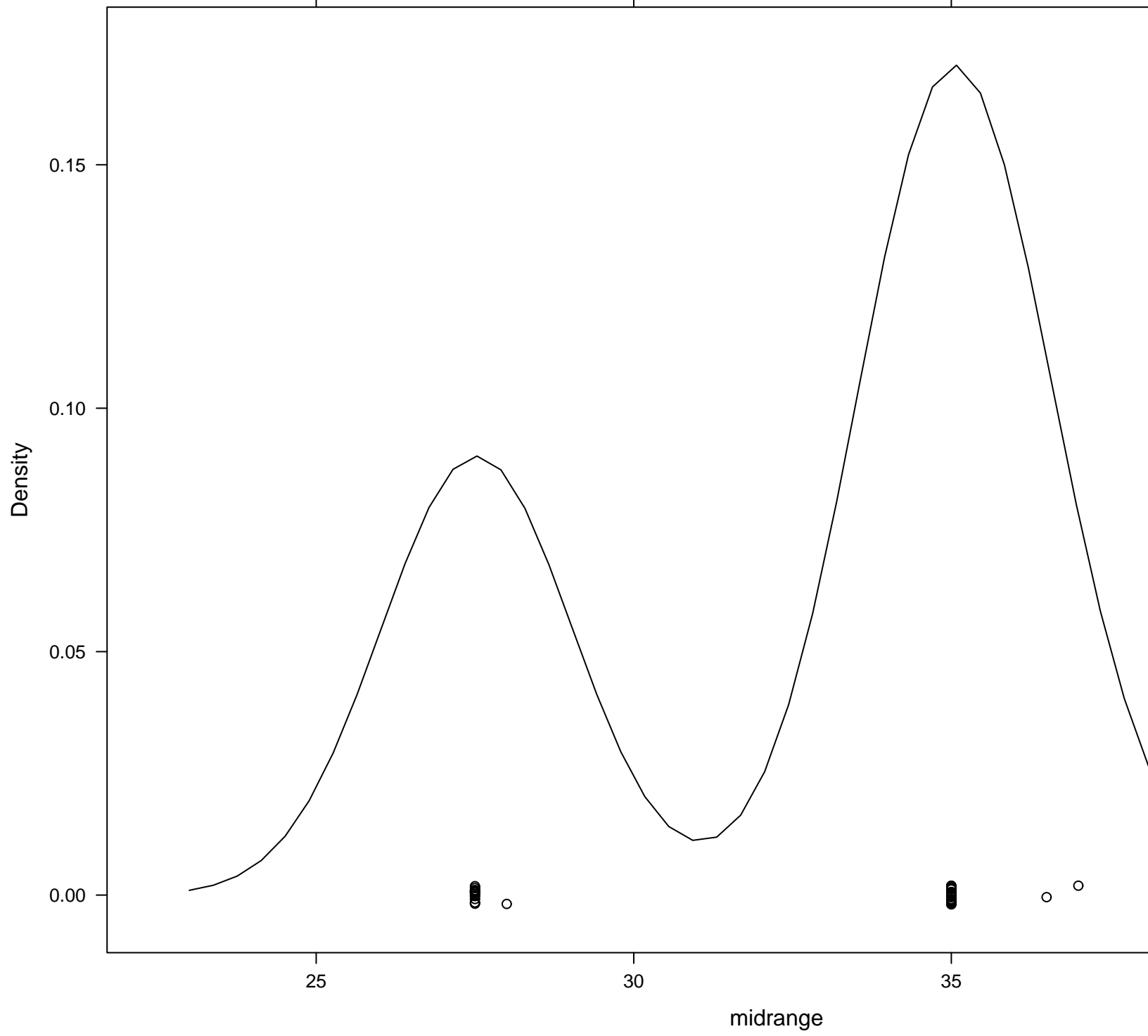
Density Plot
