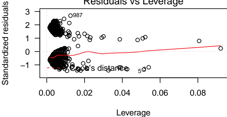
Residuals vs Leverage
