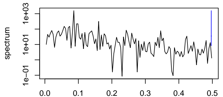
Random
