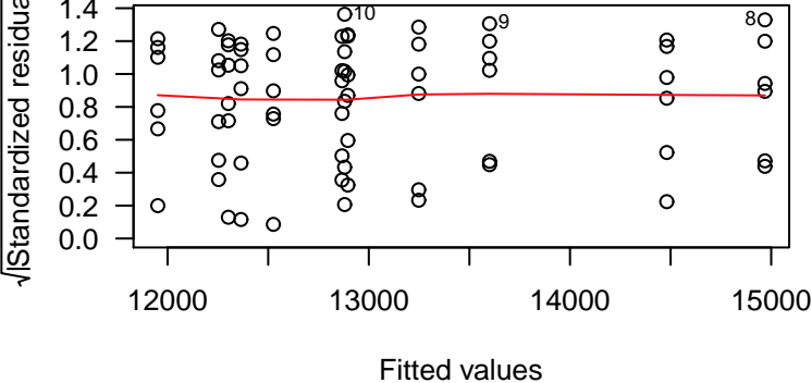
Scale-Location
