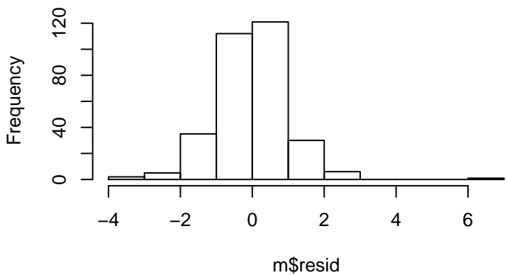
Residual Histogram
