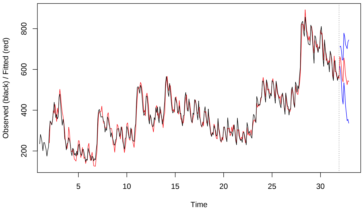
Extrapolation Fit of Exponential Smoothing
