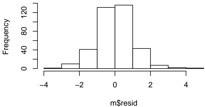
Residual Histogram
