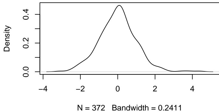
Residual Kernel Density
