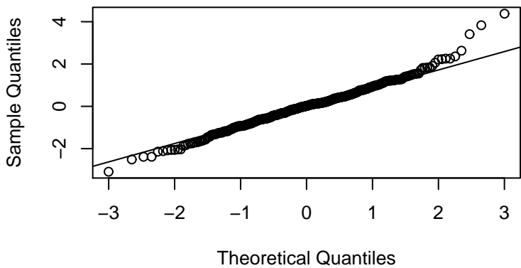
Residual Normal QQ Plot
