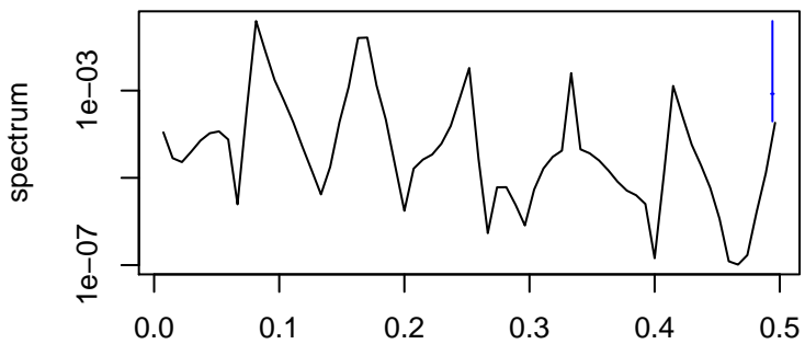
Seasonal
