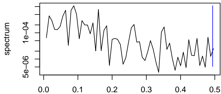
Random
