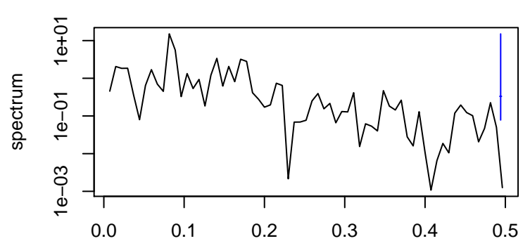
Standardized Residuals
