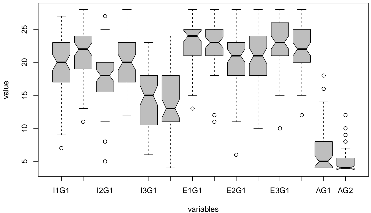
Notched Boxplots: gender 1 + 2
