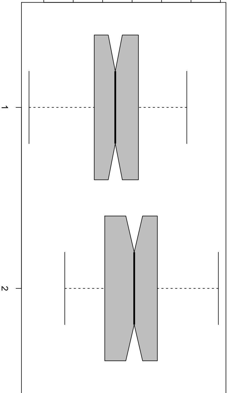
Notched Boxplots
