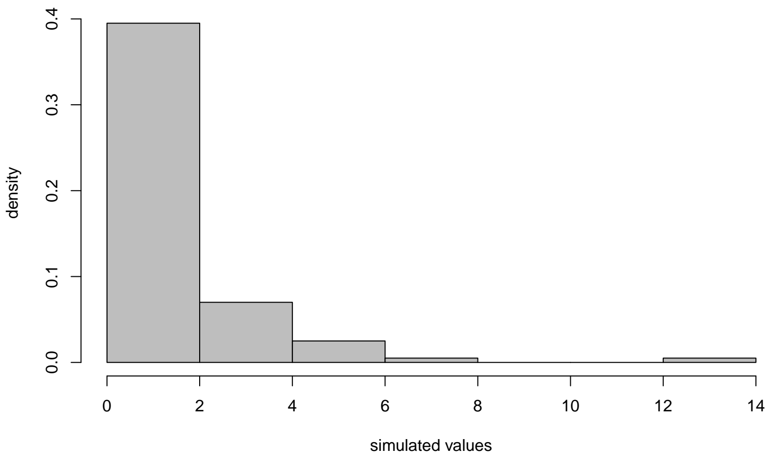
Histogram of 1st simulated series
